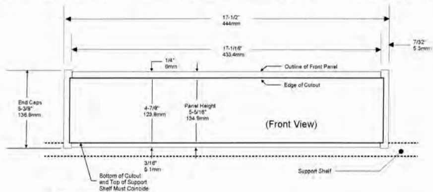
Front View of the MA6450 custom installed
