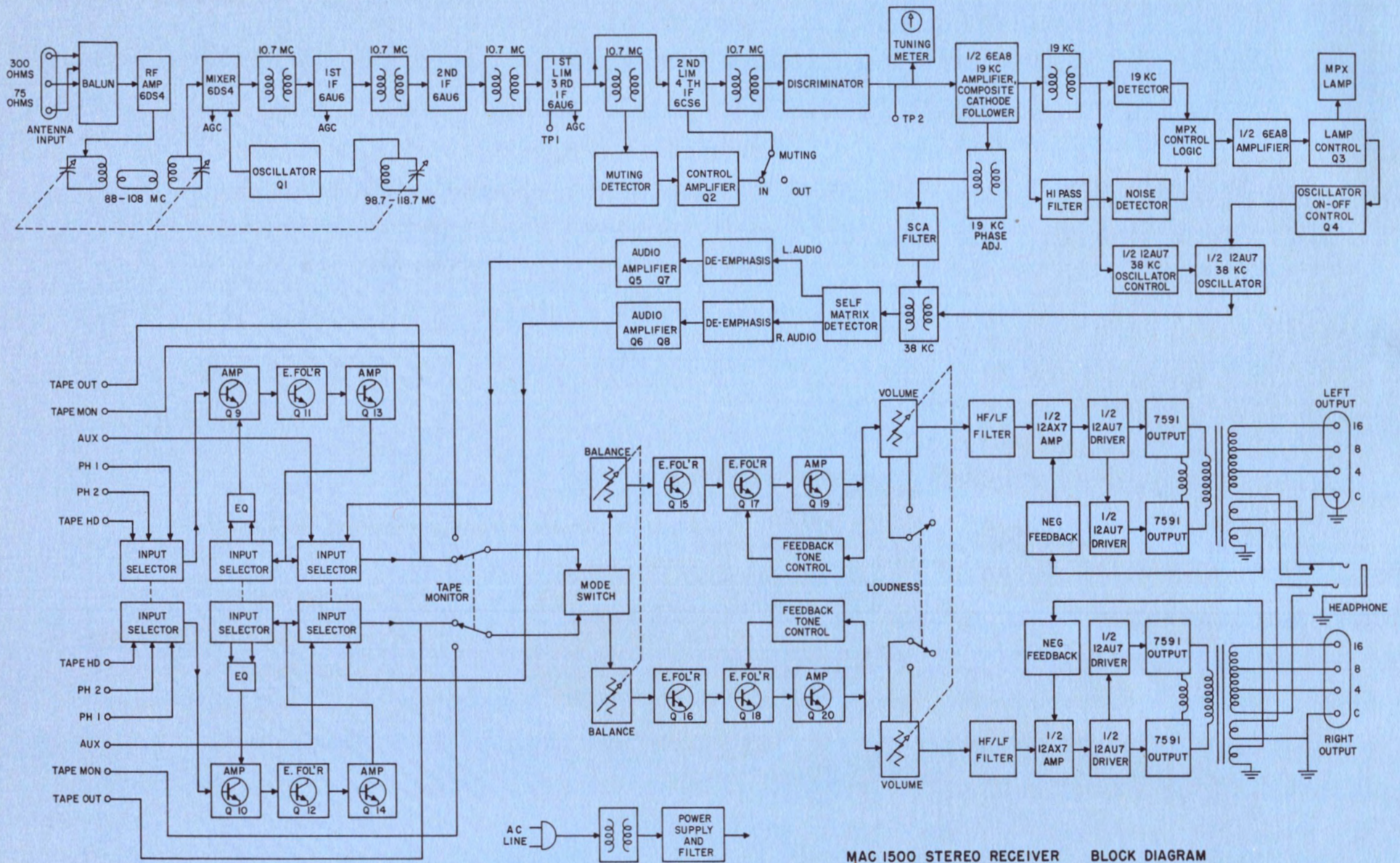
MAC 1500 STEREO RECEIVER BLOCK DIAGRAM
