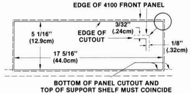
Fig. 1 Custom Cabinet Front Panel Cutout.
