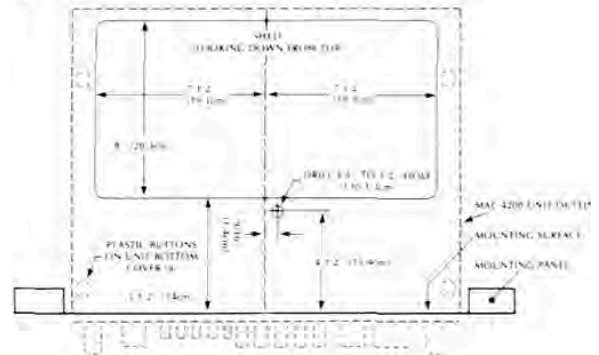
Fig. 2 Custom Cabinet Shell Mounting Cutout
