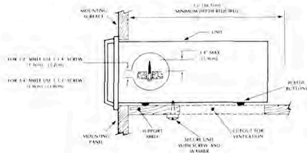
Fig. 3 MAC 4200 Custom Mounting Profile
