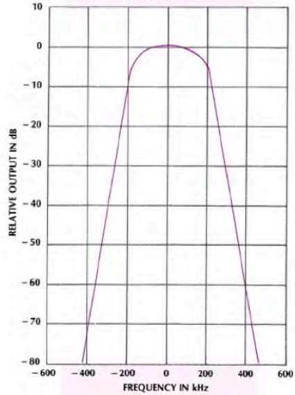
FM SELECTIVITY
