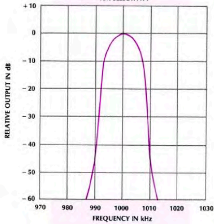
AM SELECTIVITY
