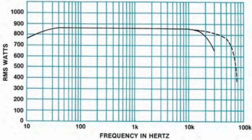
POWER OUTPUT VS FREQUENCY MONO, 8 OHM LOAD
