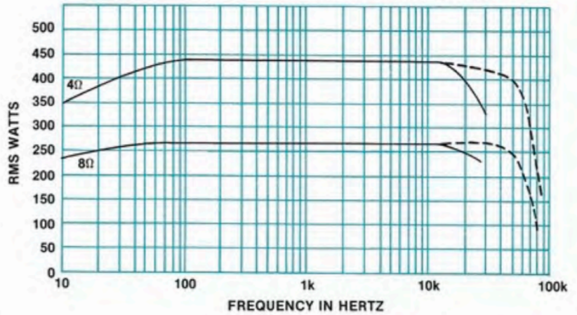
POWER OUTPUT VS FREQUENCY STEREO, BOTH CHANNELS OPERATING
