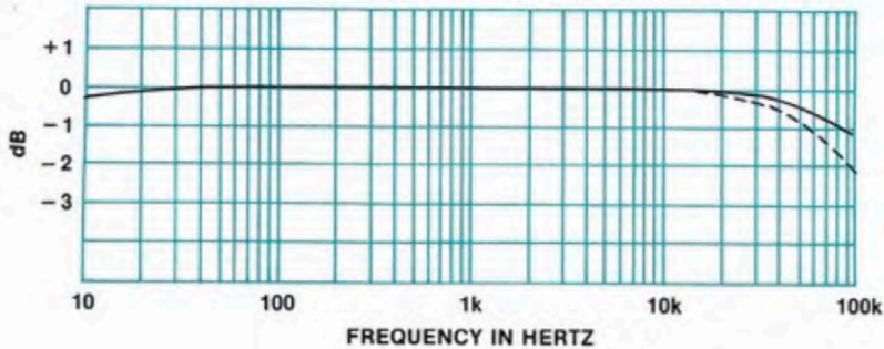
FREQUENCY RESPONSE AT 1 WATT OUTPUT
