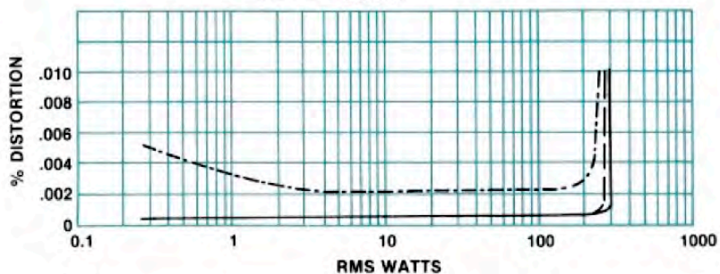
HARMONIC DISTORTION* VS POWER OUTPUT 8 OHM LOAD - - - - 20 Hz ——— 1 kHz - - - - 20 kHz
