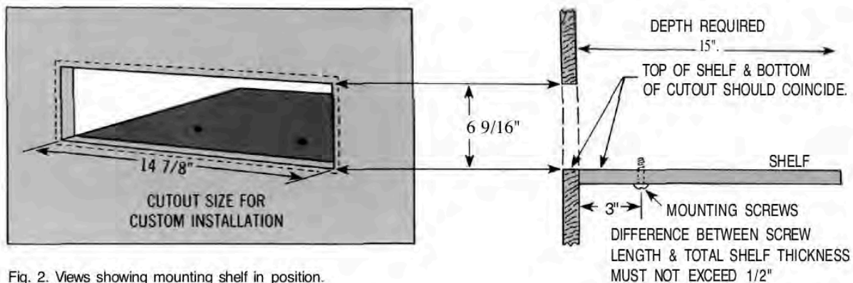
Fig. 2. Views showing mounting shelf in position.
