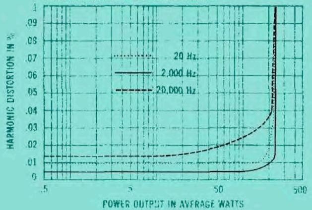
HARMONIC DISTORTION VS. POWER OUTPUT
