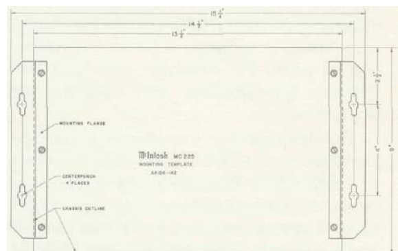
Fig. 4 Bottom of MC225 with mounting flanges attached.
