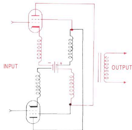
Fig. 2—Representation of McIntosh output circuit.
