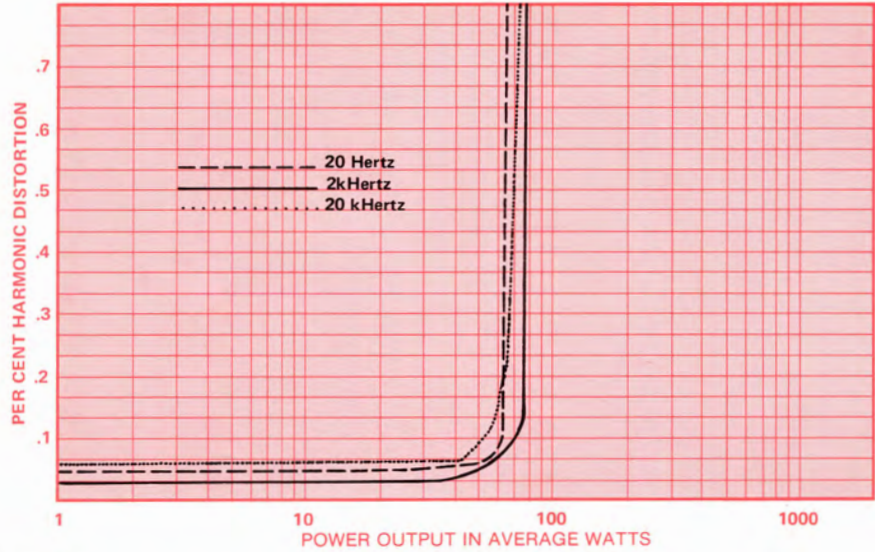
Harmonic Distortion versus Power
