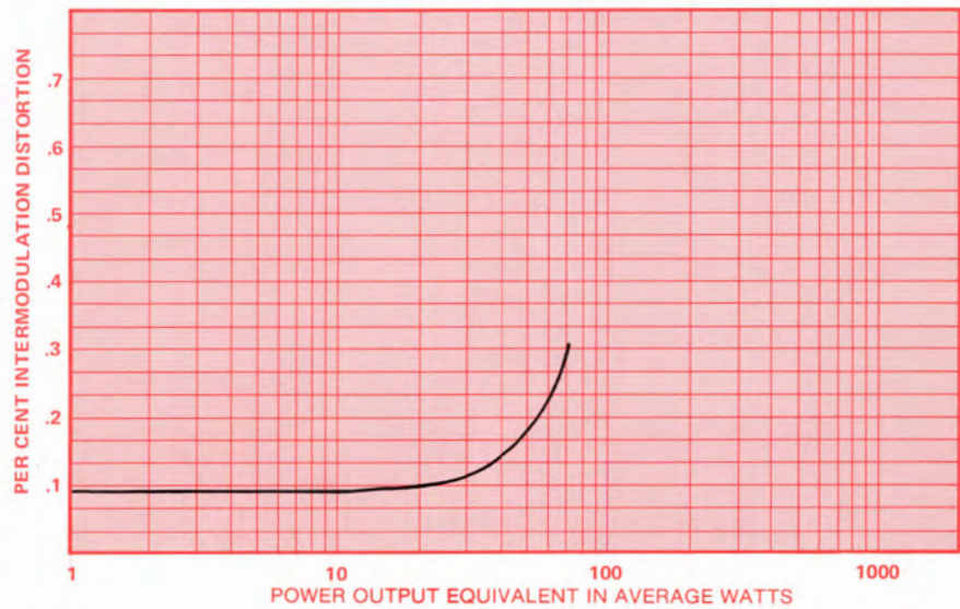
Equivalent Power Output versus Intermodulation Distortion
