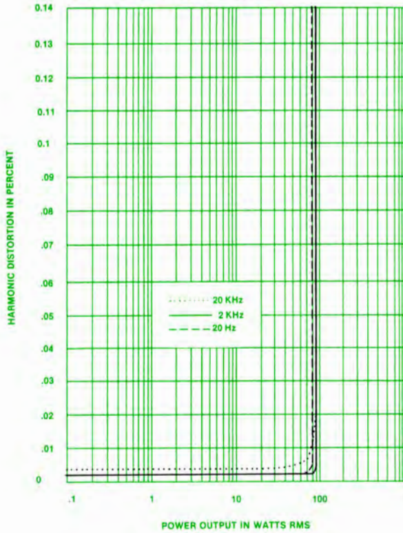
HARMONIC DISTORTION VS POWER OUTPUT RL = 8 OHMS, BOTH CHANNELS OPERATING
