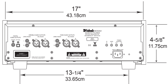
Rear View of the MCD201
