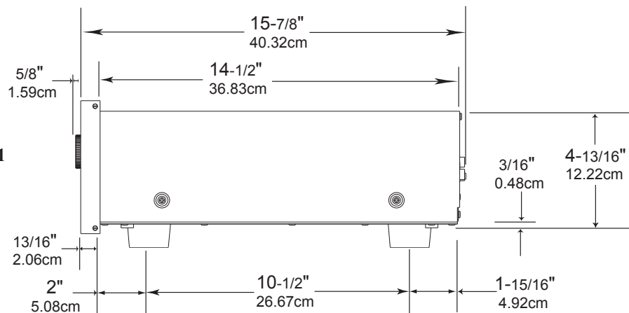
Side View of the MCD201
