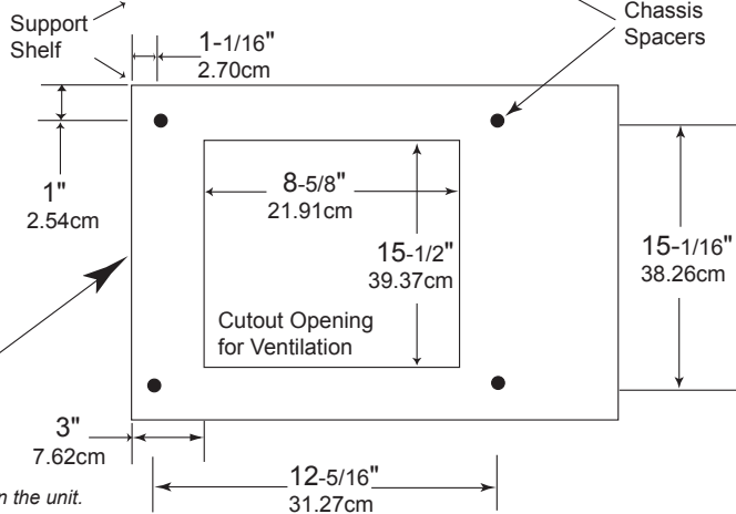
MCD201 Bottom View in Custom Cabinet
