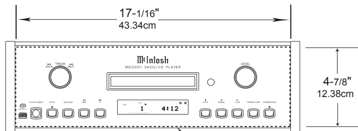
MCD201 Front Panel Custom Cabinet Cutout
