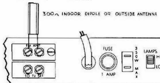
Fig. 18—Connection for 300 ohm antenna.
