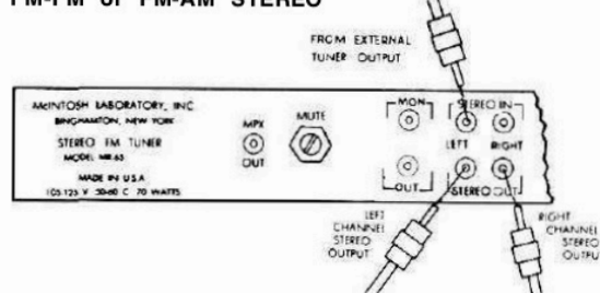
Fig. 17—Connection for external tuner for stereo.
