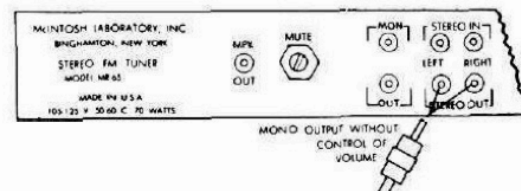
Fig. 14—Monophonic output without volume control.
