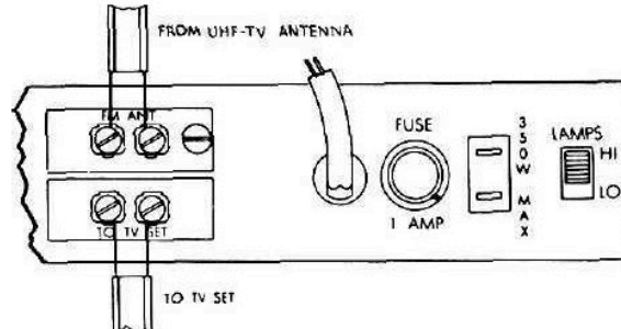
Fig. 20—Connections for sharing a VHF-TV antenna.
