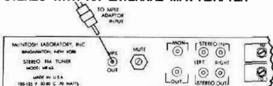
Fig. 16—Connections for an external MPX adapter.
