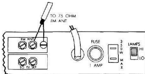
Fig. 19—Connections for a 75 ohm antenna.
