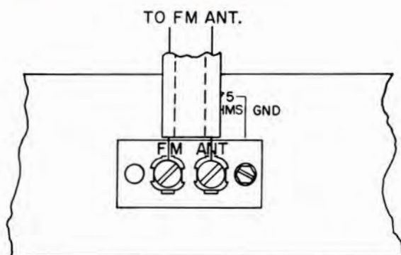
Figure 12. Connection of 300 Ohm Indoor Dipole FM Antenna
