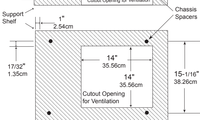
MR85 Bottom View in Custom Cabinet
