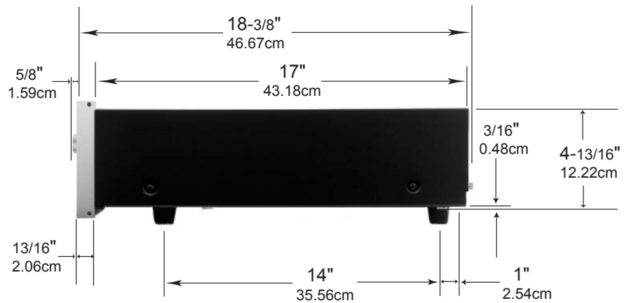
Side View of the MR85
