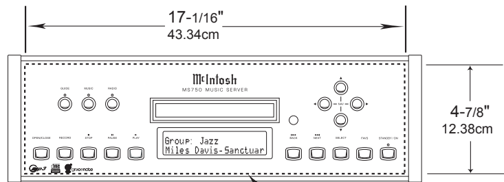
MS750 Front Panel Custom Cabinet Cutout
