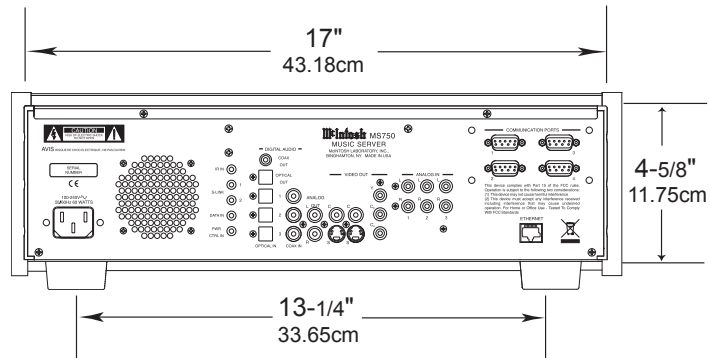
Rear View of the MS750
