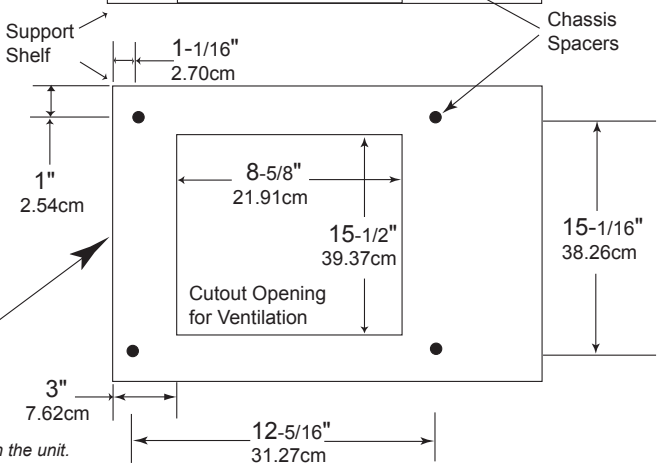
MS750 Bottom View in Custom Cabinet
