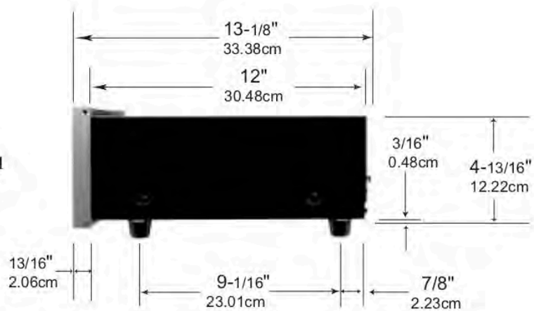
Side View of the MVP851
