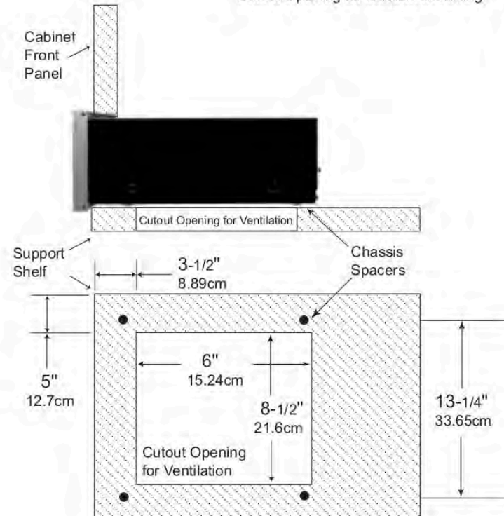
Cutout Opening for Custom Mounting
