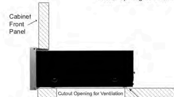
MVP861 Side View in Custom Cabinet
