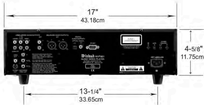
Rear View of the MVP861
