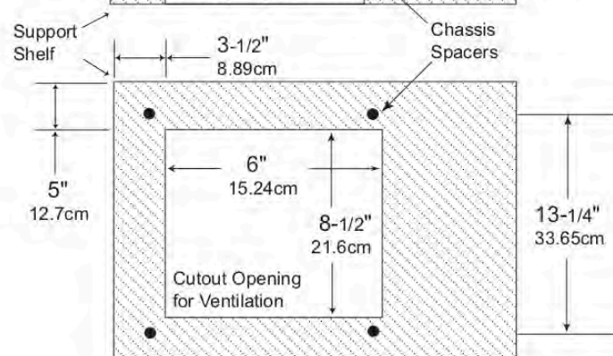
MVP861 Bottom View in Custom Cabinet
