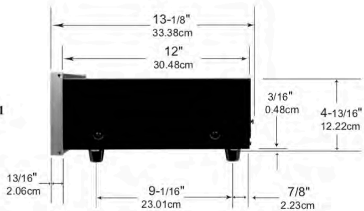
Side View of the MVP861
