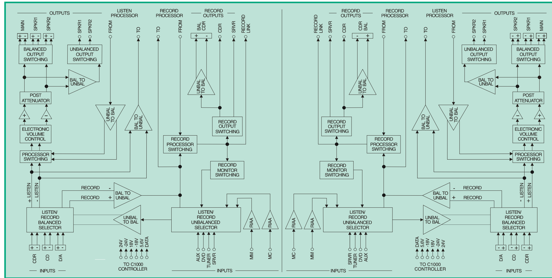
C1000 Preamplifier
