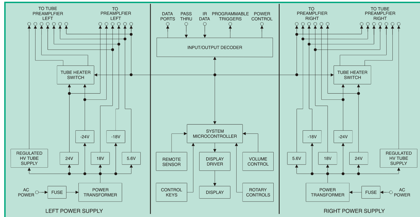
C1000 Controller
