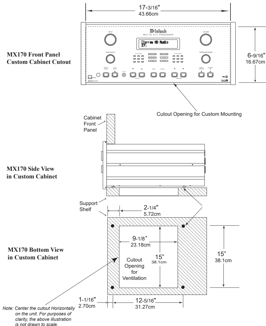
Figure 02– Custom cutout dimensions
