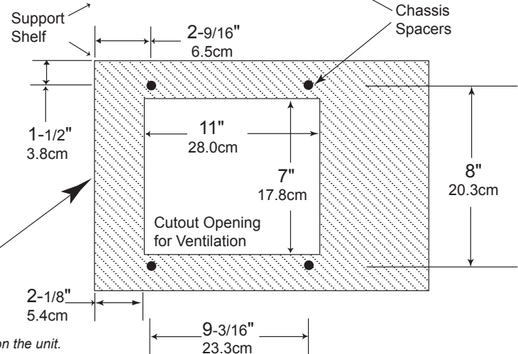
MCT80 Bottom View in Custom Cabinet
