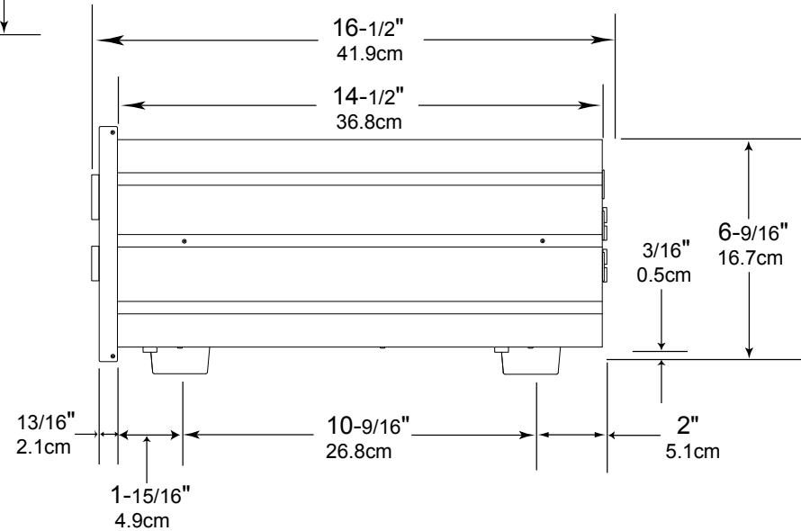
Side View of the MX160
