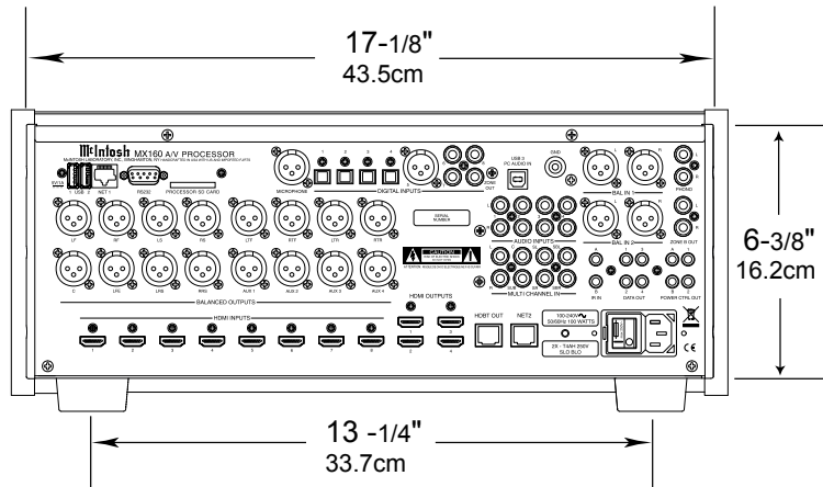
Rear View of the MX160
