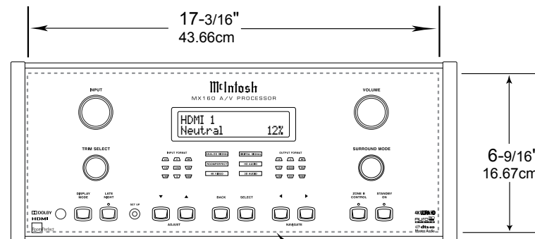
MX160 Front Panel Custom Cabinet Cutout
