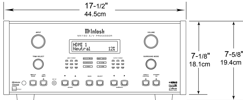
Front View of the MX160
