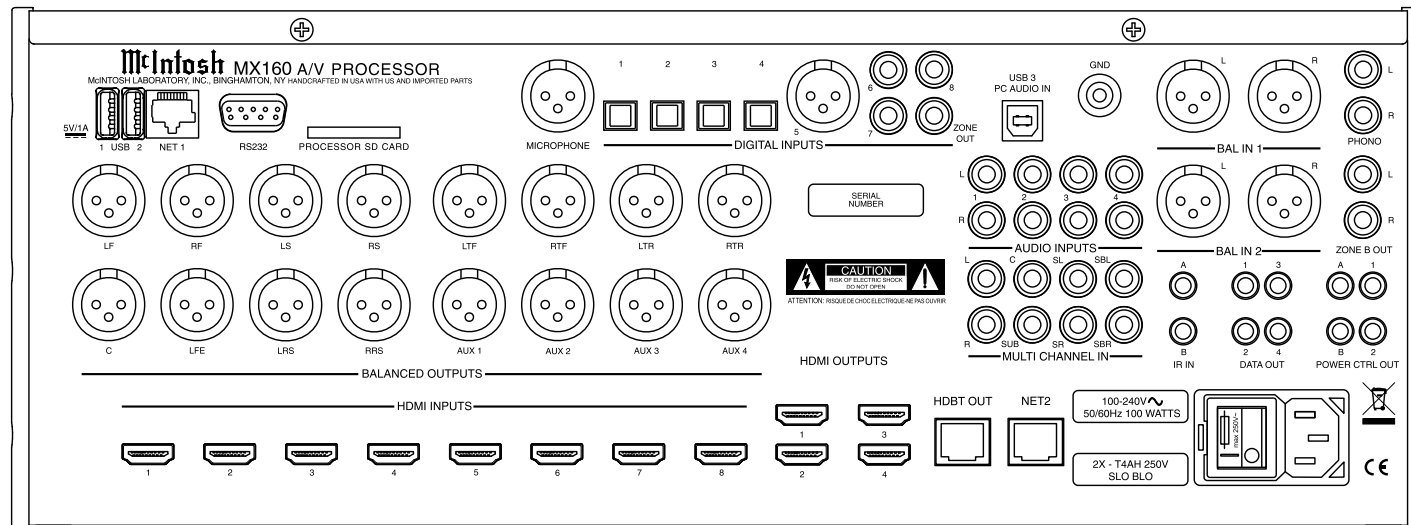
MX160 A/V Processor Rear Panel
