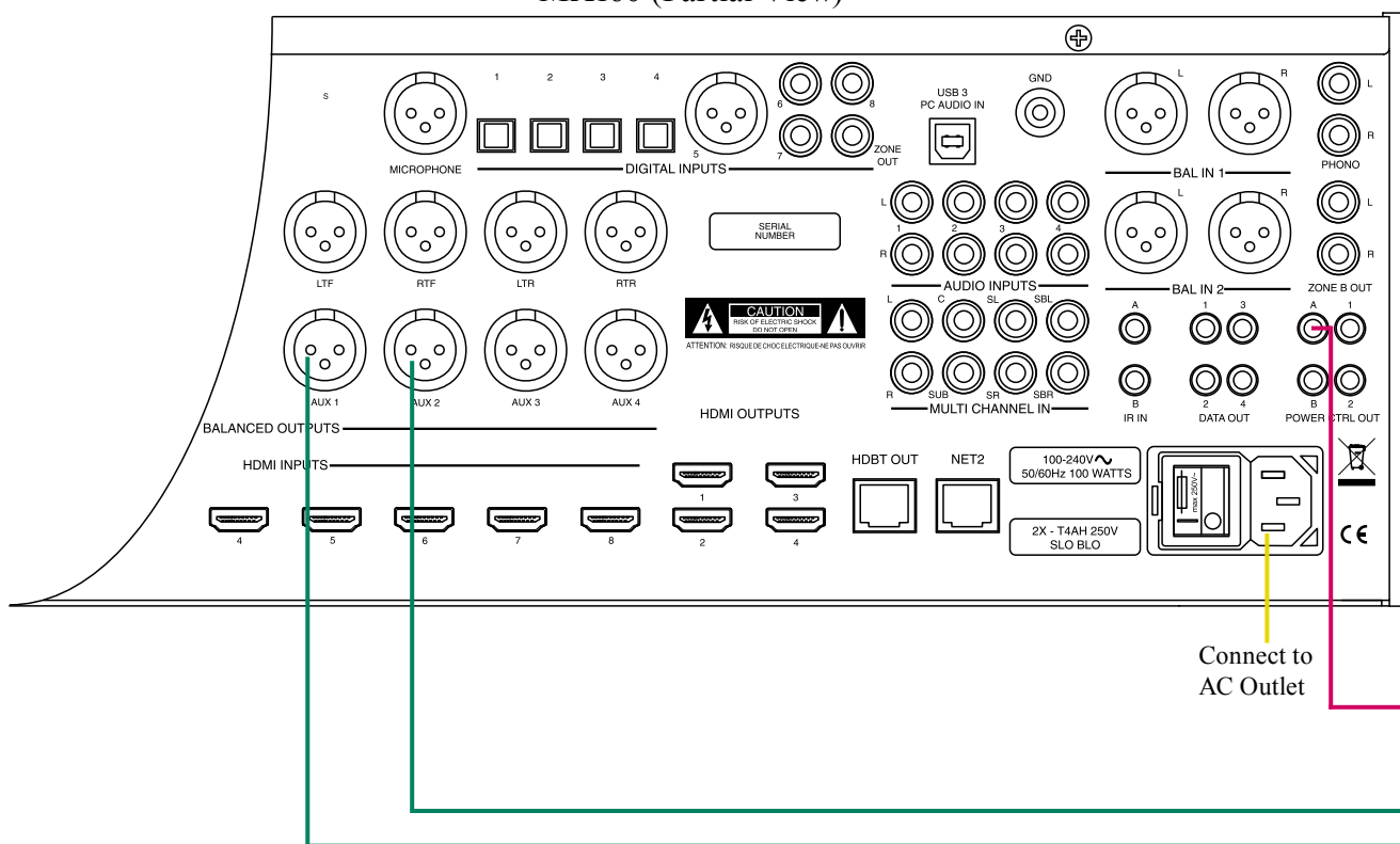
MX160 (Partial View)
